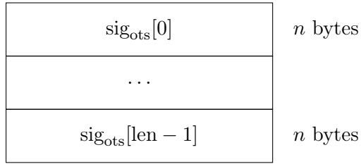
Figure 9: WOTS + Signature data format.
